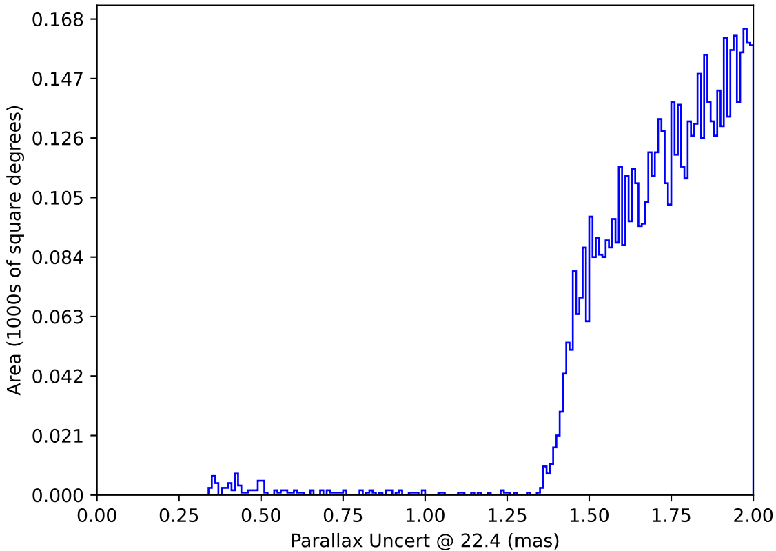
mw_roll_all_v3.3_10yrs : Parallax Uncert @ 22.4
