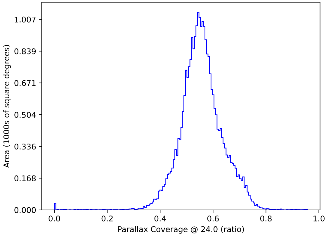
mw_roll_all_v3.3_10yrs : Parallax Coverage @ 24.0
