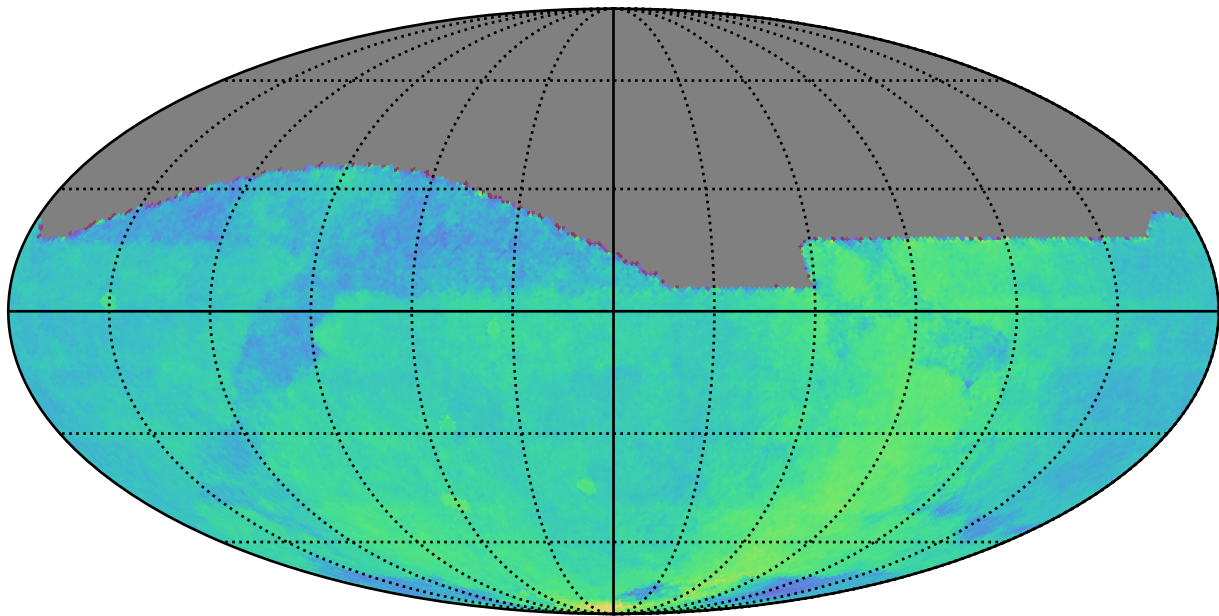
mw_roll_all_v3.3_10yrs : Parallax Coverage @ 22.4
