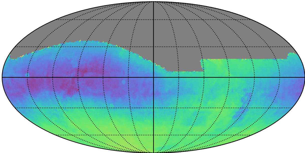
mw_roll_all_v3.3_10yrs : Parallax-DCR degeneracy @ 24.0
