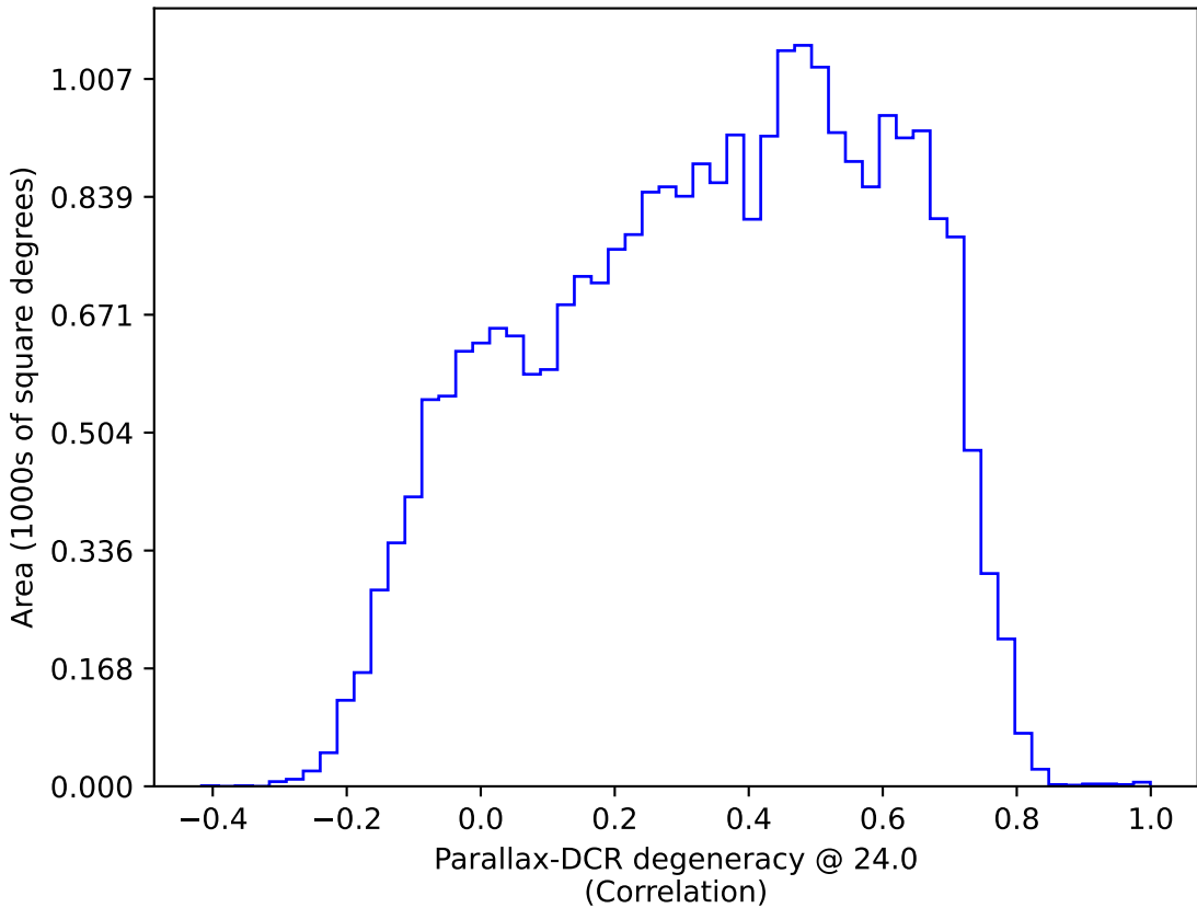
mw_roll_all_v3.3_10yrs : Parallax-DCR degeneracy @ 24.0
