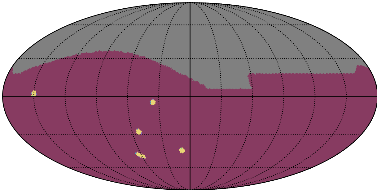
mw_roll_all_v3.3_10yrs : NumberOfQuickRevisits
