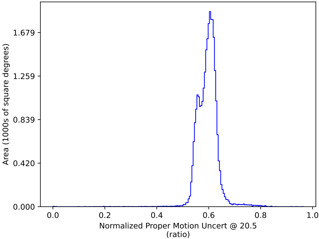
mw_roll_all_v3.3_10yrs : Normalized Proper Motion Uncert @ 20.5
