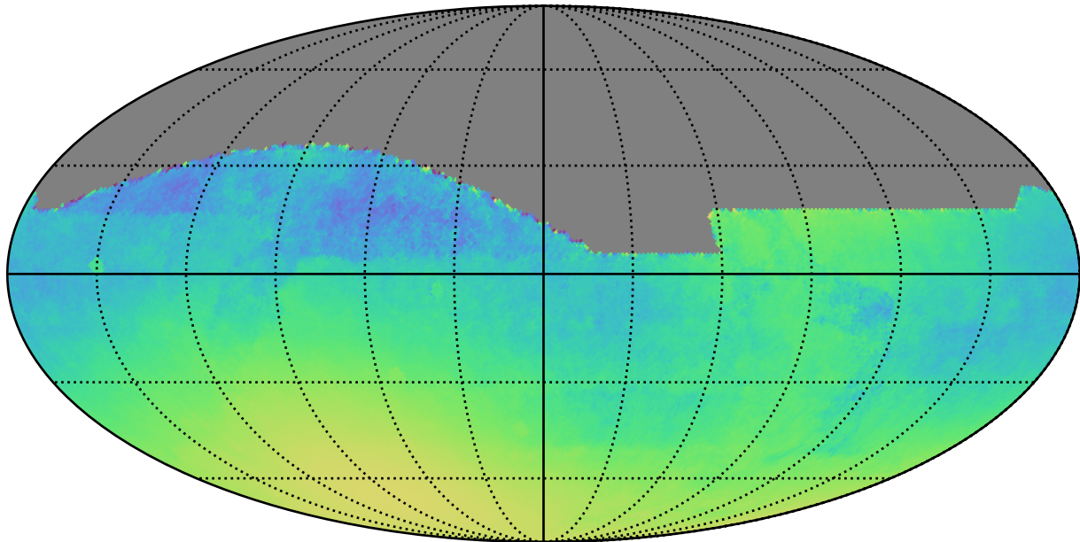
mw_roll_all_v3.3_10yrs : Normalized Parallax Uncert @ 24.0
