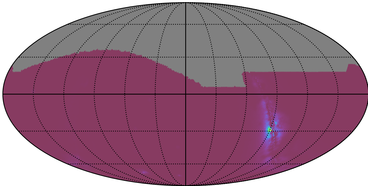
mw_roll_all_v3.3_10yrs : NlcPoints
