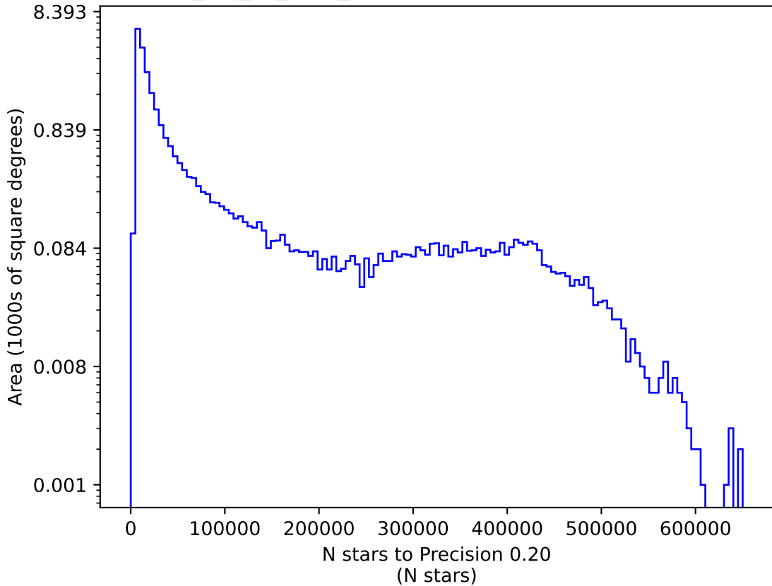
mw_roll_all_v3.3_10yrs z: N stars to Precision 0.20
