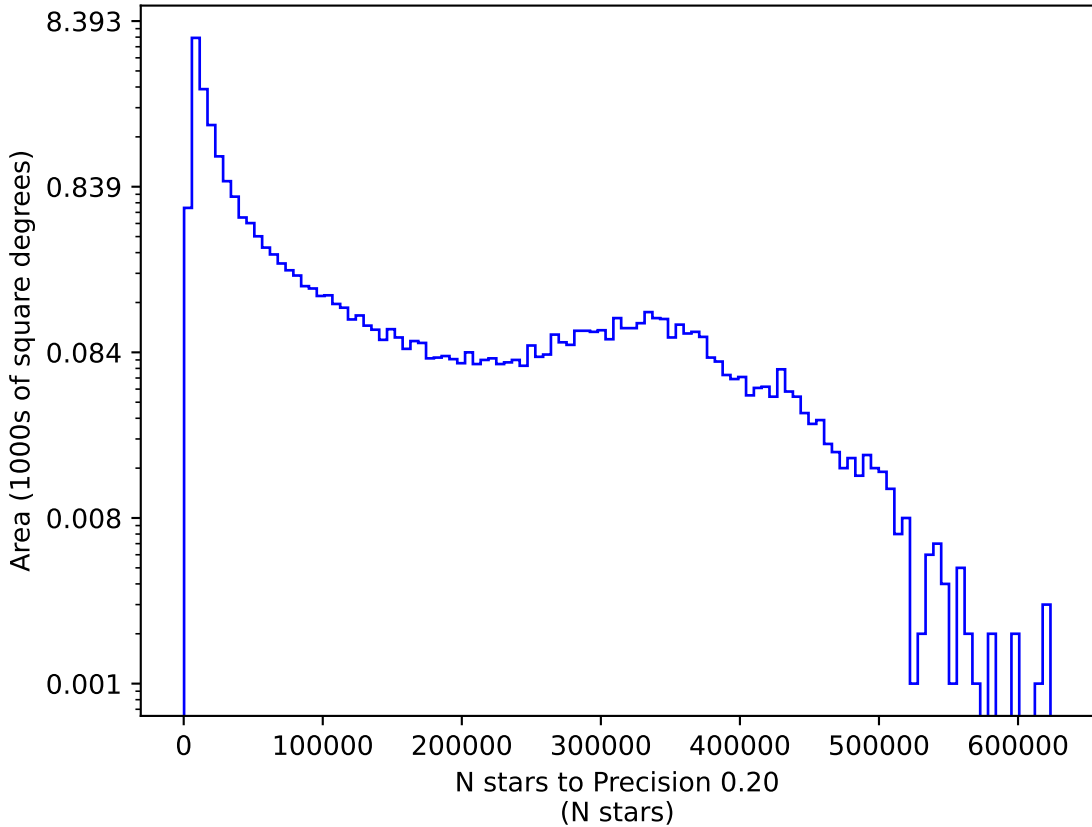
mw_roll_all_v3.3_10yrs y: N stars to Precision 0.20
