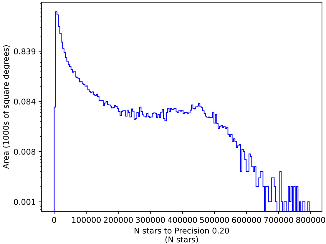
mw_roll_all_v3.3_10yrs r: N stars to Precision 0.20
