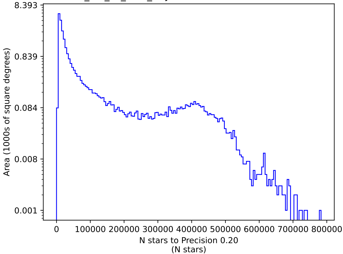
mw_roll_all_v3.3_10yrs i: N stars to Precision 0.20
