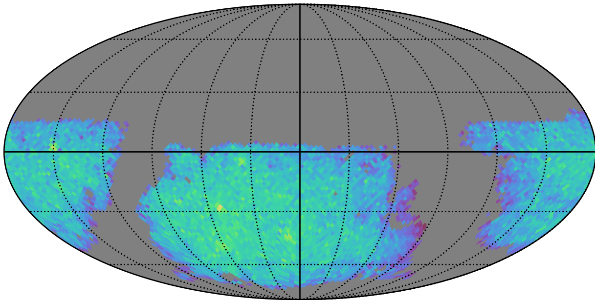
mw_roll_all_v3.3_10yrs gi: LVDwarfs
