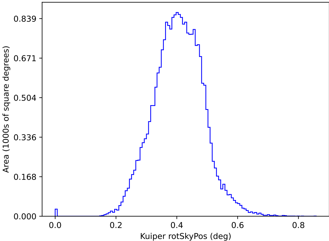
mw_roll_all_v3.3_10yrs y: Kuiper rotSkyPos
