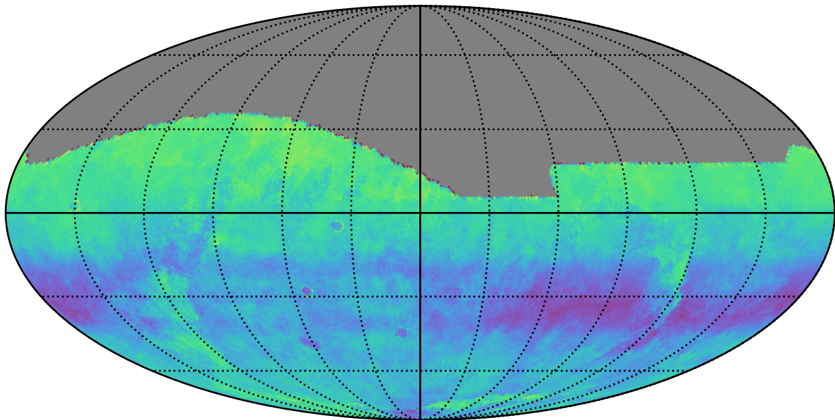
mw_roll_all_v3.3_10yrs r: Kuiper rotSkyPos
