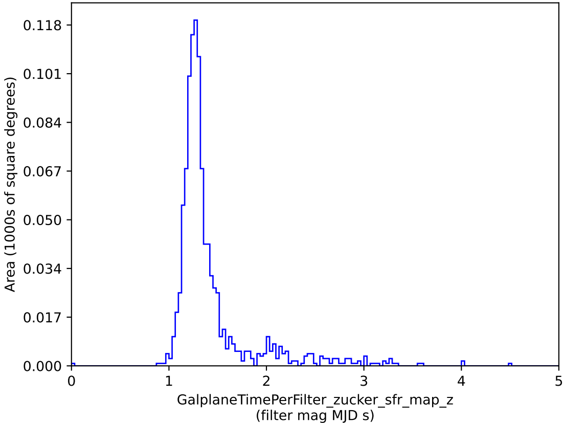
mw_roll_all_v3.3_10yrs : GalplaneTimePerFilter_zucker_sfr_map_z
