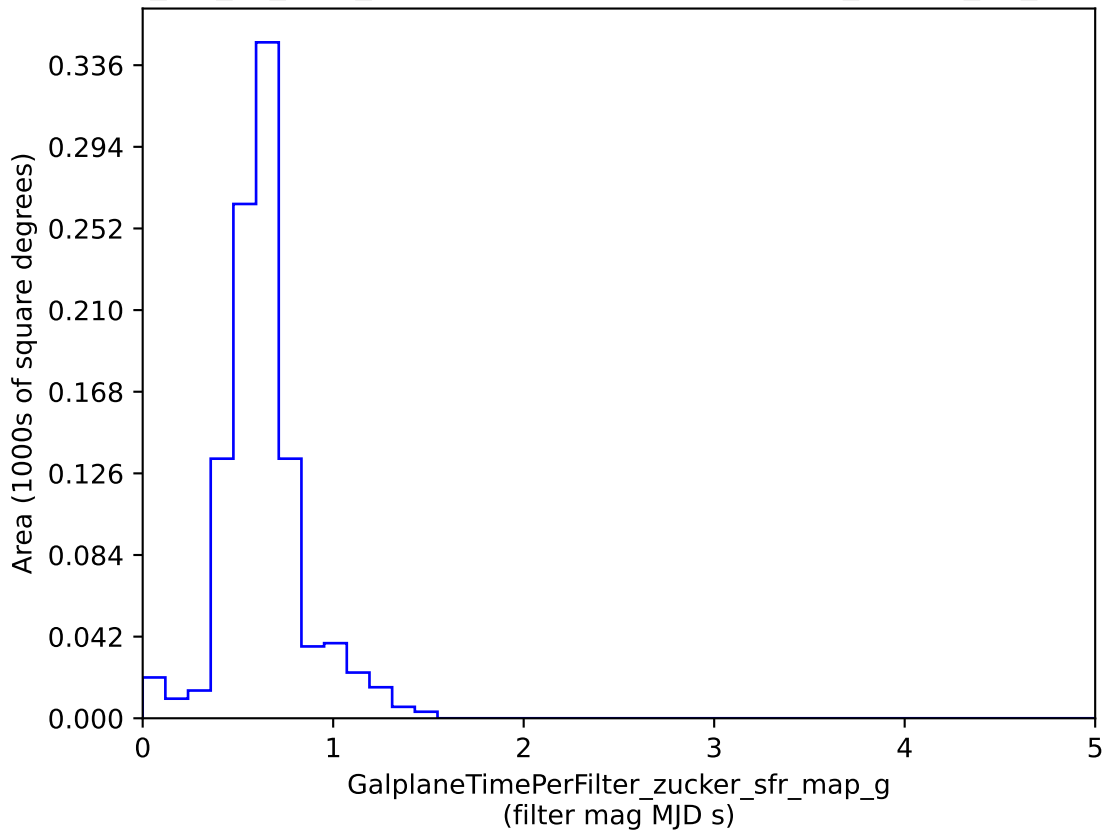
mw_roll_all_v3.3_10yrs : GalplaneTimePerFilter_zucker_sfr_map_g
