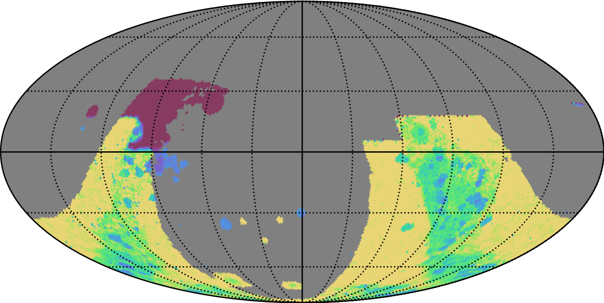
mw_roll_all_v3.3_10yrs : GalplaneTimePerFilter_combined_map_y
