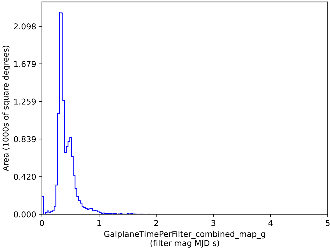
mw_roll_all_v3.3_10yrs : GalplaneTimePerFilter_combined_map_g
