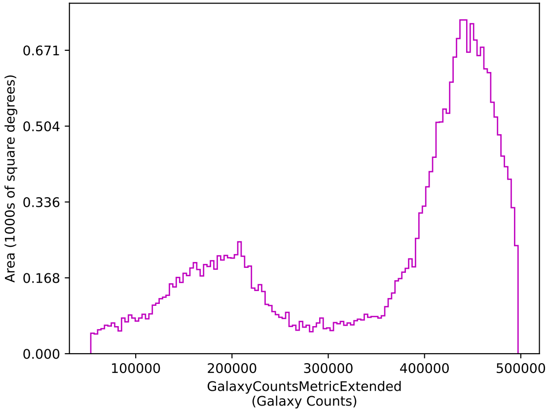
mw_roll_all_v3.3_10yrs z: GalaxyCountsMetricExtended
