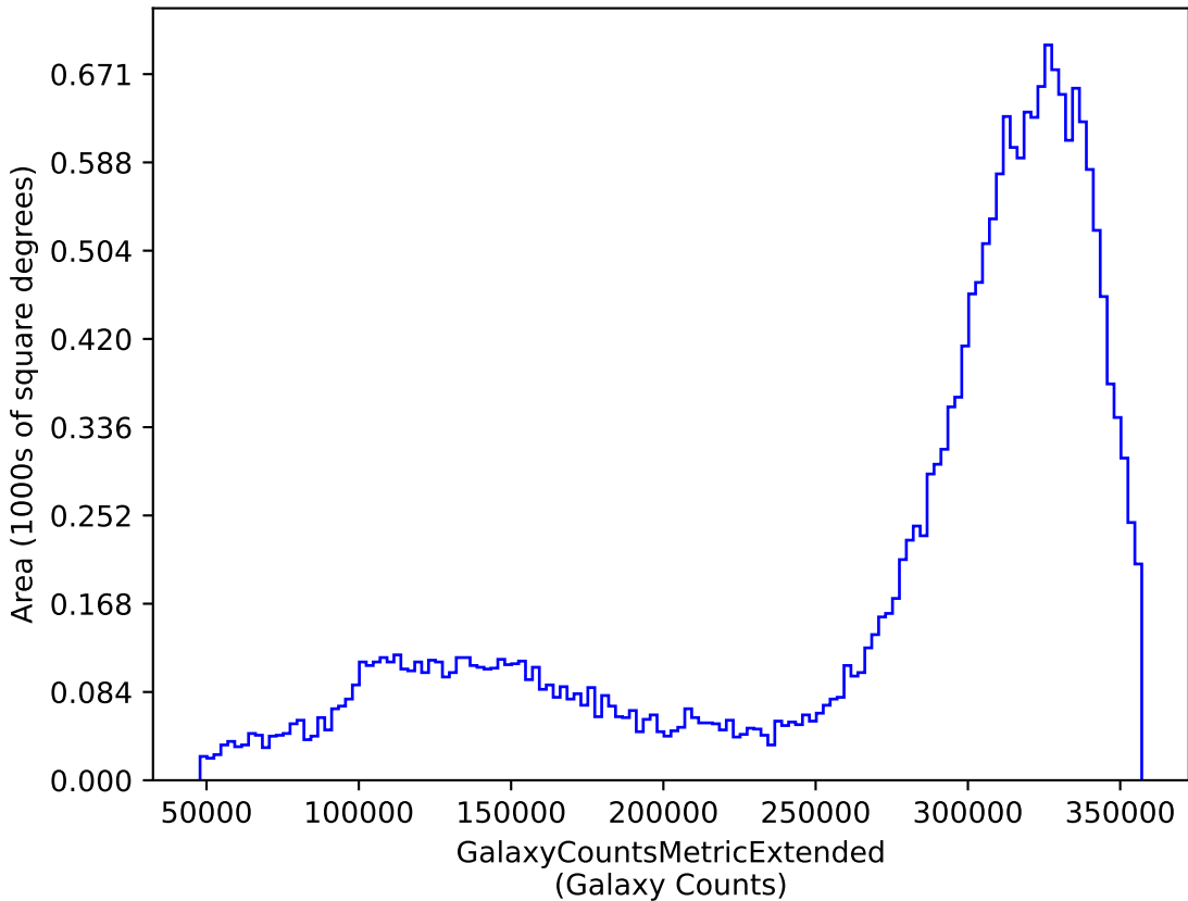
mw_roll_all_v3.3_10yrs y: GalaxyCountsMetricExtended
