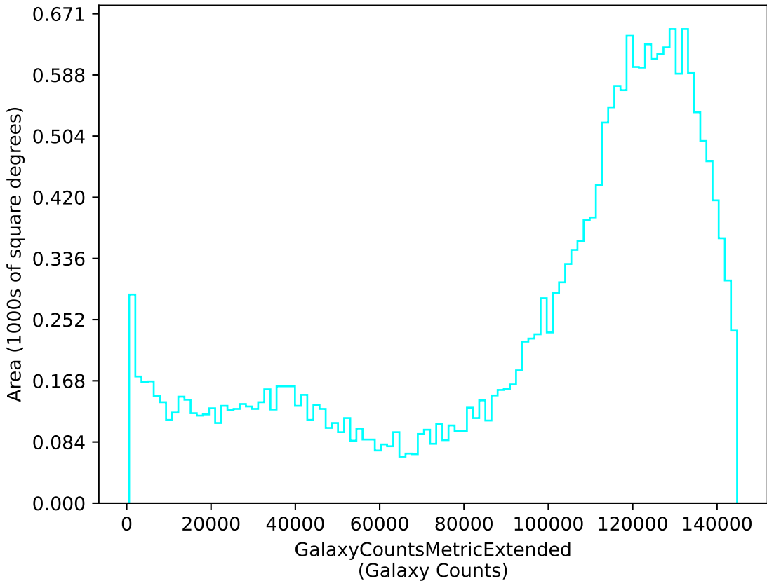
mw_roll_all_v3.3_10yrs u: GalaxyCountsMetricExtended
