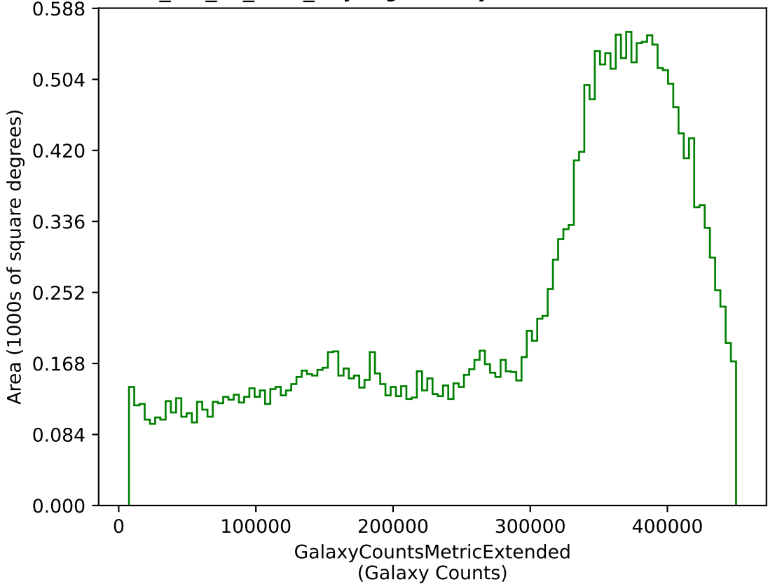
mw_roll_all_v3.3_10yrs g: GalaxyCountsMetricExtended
