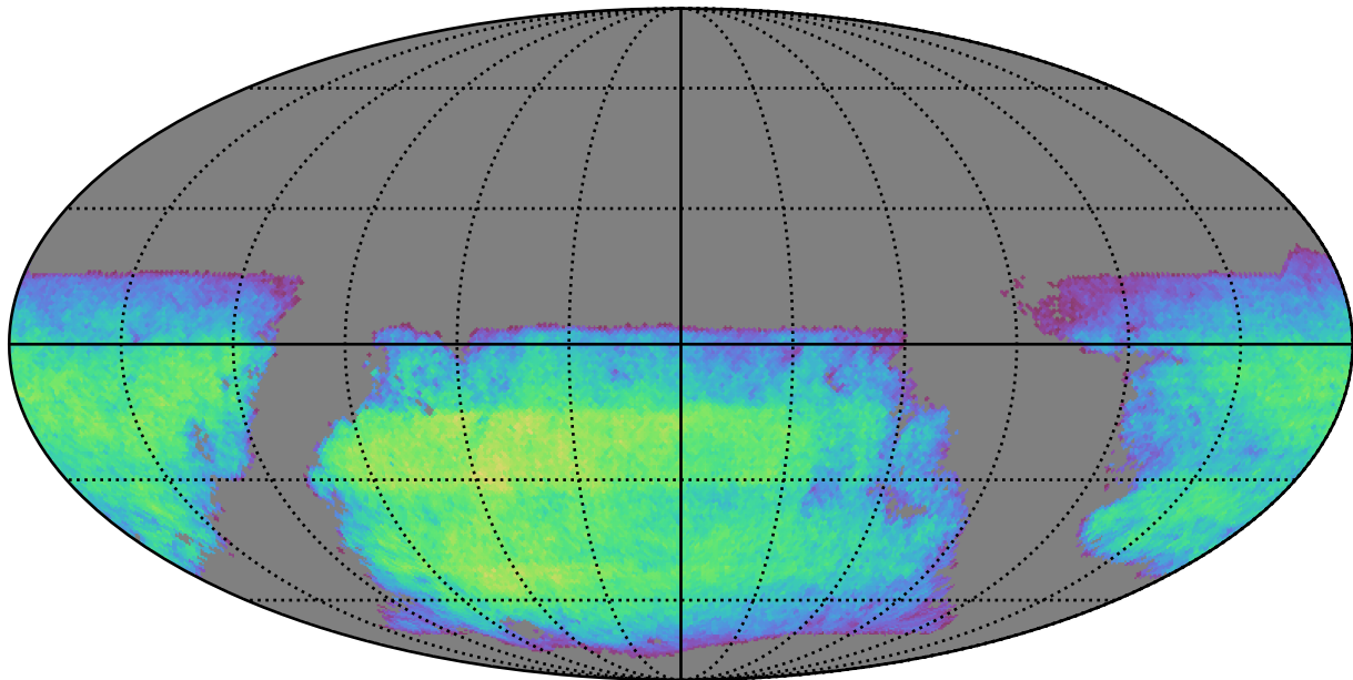
mw_roll_all_v3.3_10yrs i band non-DD year 9: ExgalM5WithCuts
