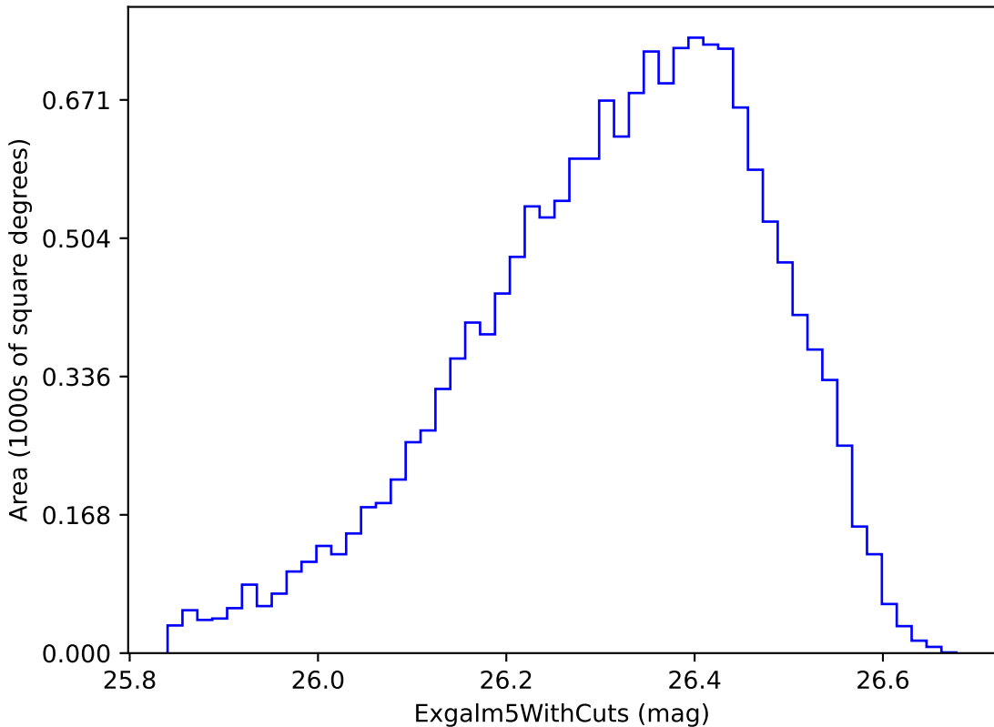
mw_roll_all_v3.3_10yrs i band non-DD year 9: ExgalM5WithCuts
