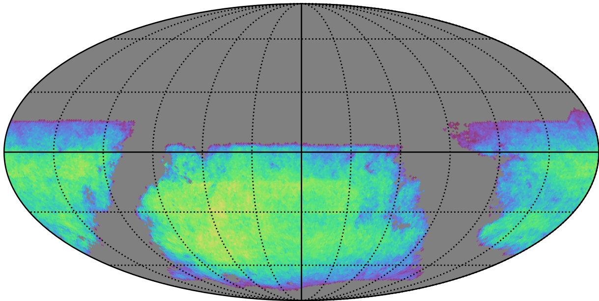
mw_roll_all_v3.3_10yrs i band non-DD year 8: ExgalM5WithCuts
