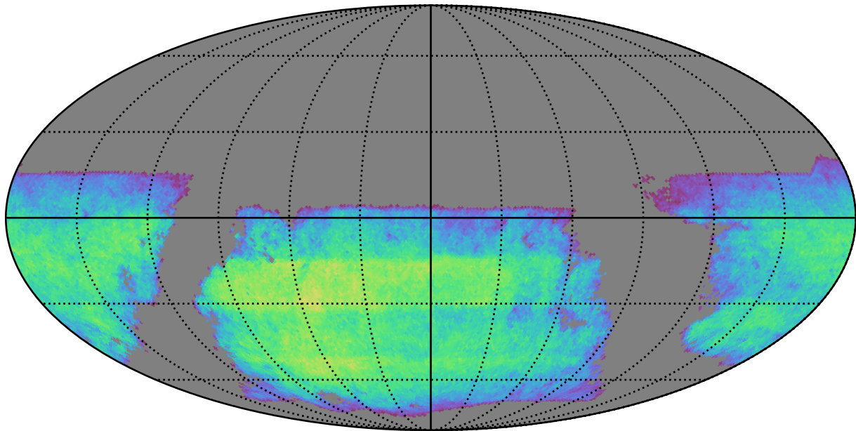
mw_roll_all_v3.3_10yrs i band non-DD year 7: ExgalM5WithCuts
