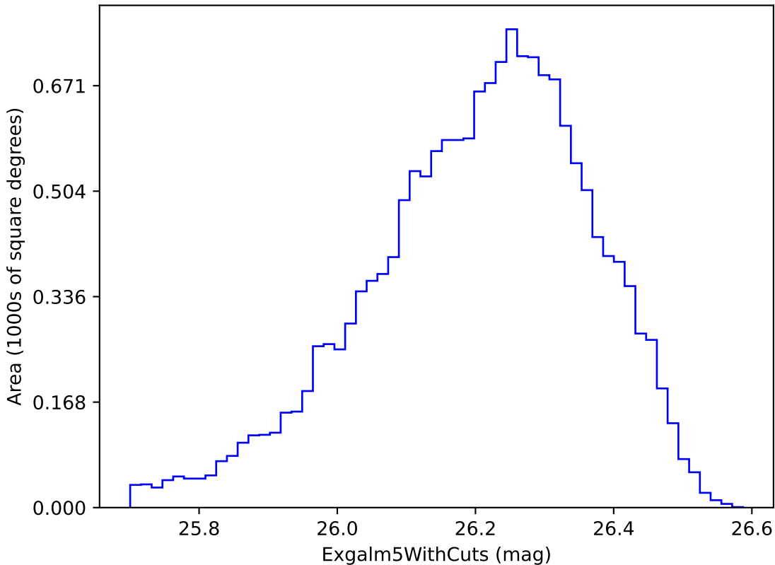
mw_roll_all_v3.3_10yrs i band non-DD year 7: ExgalM5WithCuts
