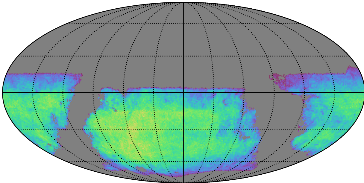
mw_roll_all_v3.3_10yrs i band non-DD year 6: ExgalM5WithCuts
