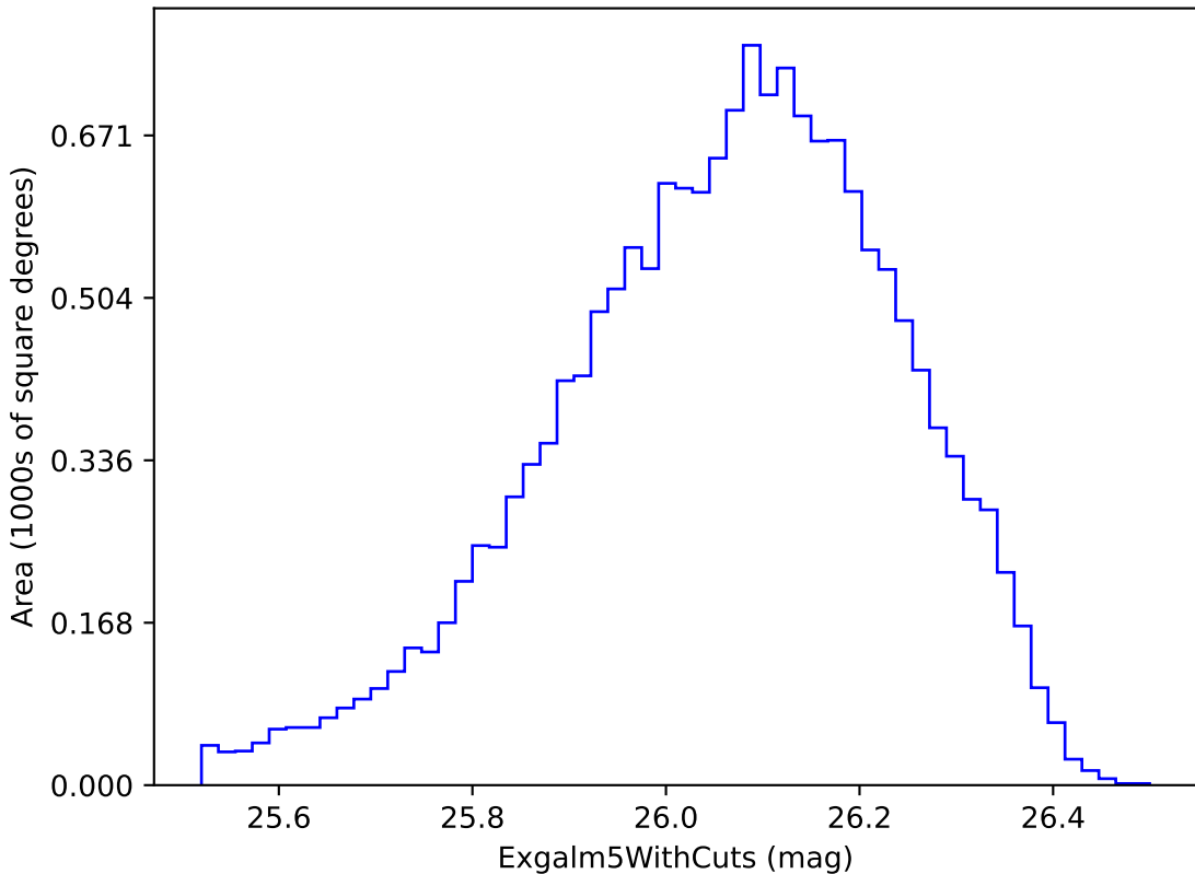
mw_roll_all_v3.3_10yrs i band non-DD year 5: ExgalM5WithCuts
