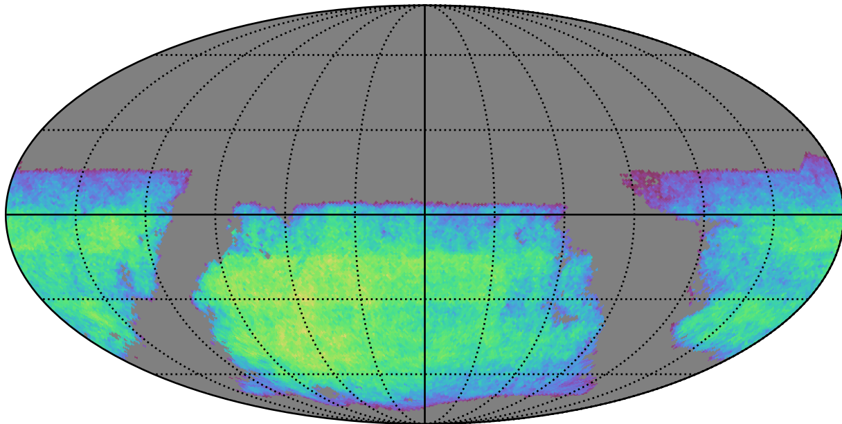
mw_roll_all_v3.3_10yrs i band non-DD year 4: ExgalM5WithCuts
