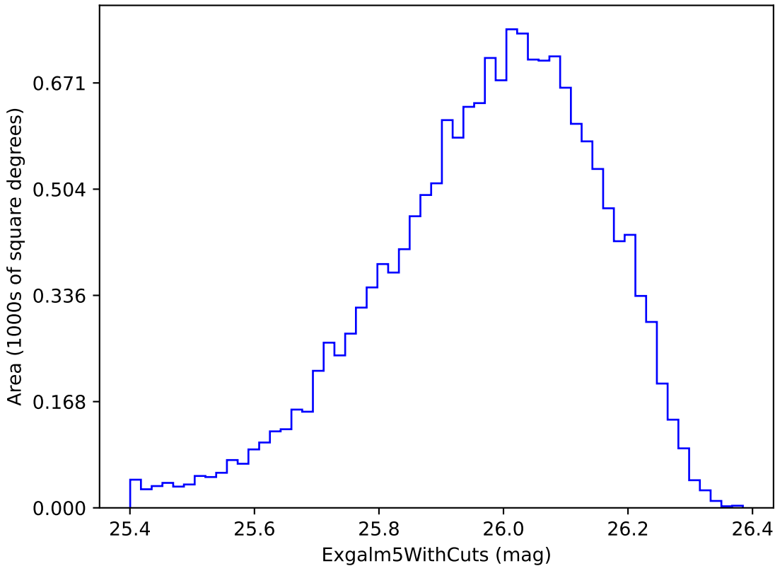
mw_roll_all_v3.3_10yrs i band non-DD year 4: ExgalM5WithCuts
