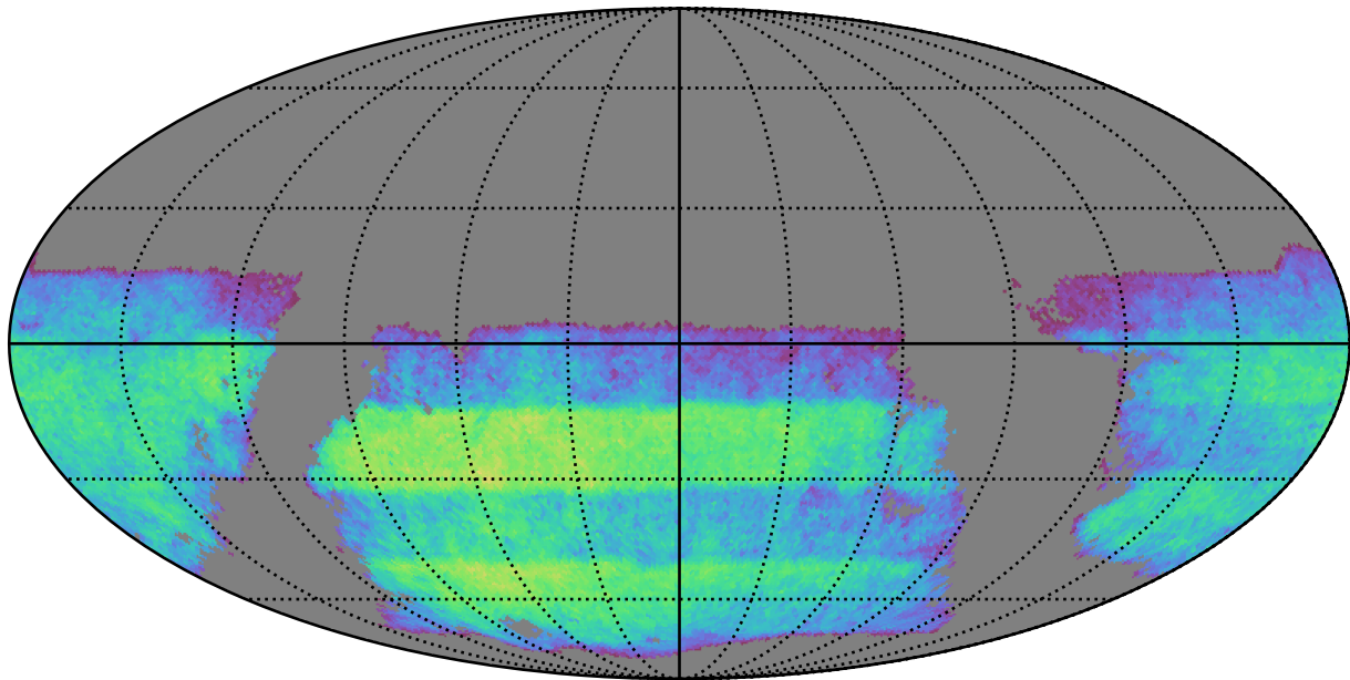
mw_roll_all_v3.3_10yrs i band non-DD year 3: ExgalM5WithCuts
