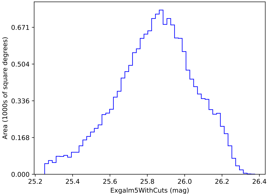
mw_roll_all_v3.3_10yrs i band non-DD year 3: ExgalM5WithCuts
