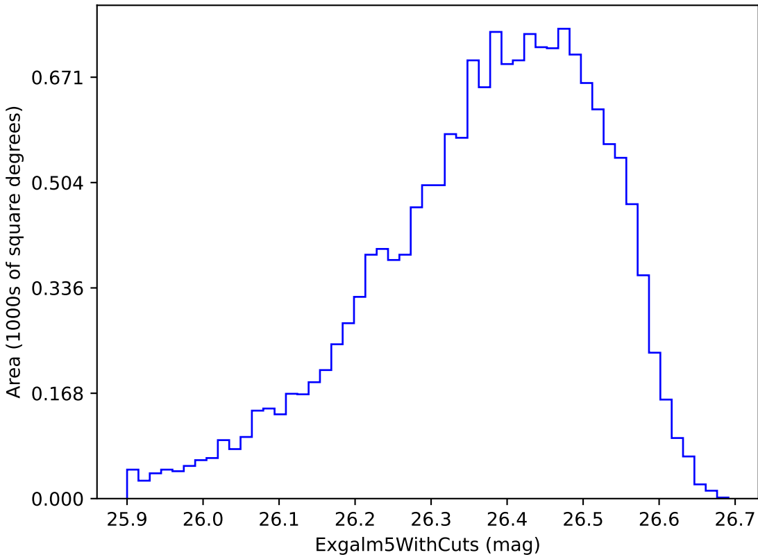
mw_roll_all_v3.3_10yrs i band non-DD year 10: ExgalM5WithCuts
