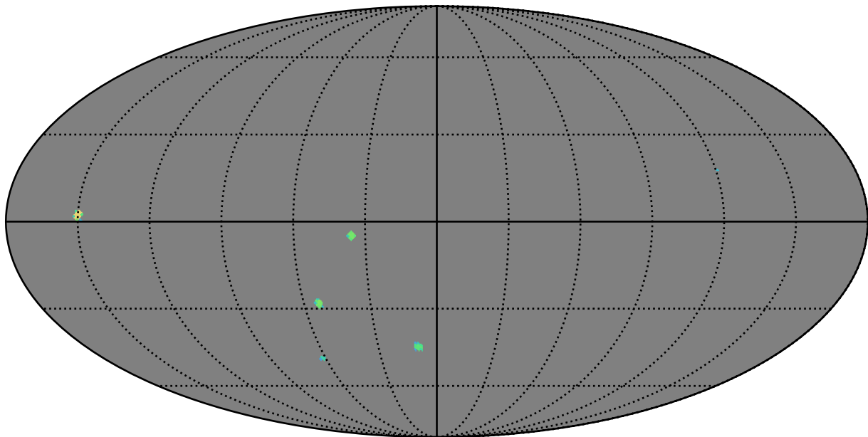
mw_roll_all_v3.3_10yrs z band: AGN_TimeLag_5_days
