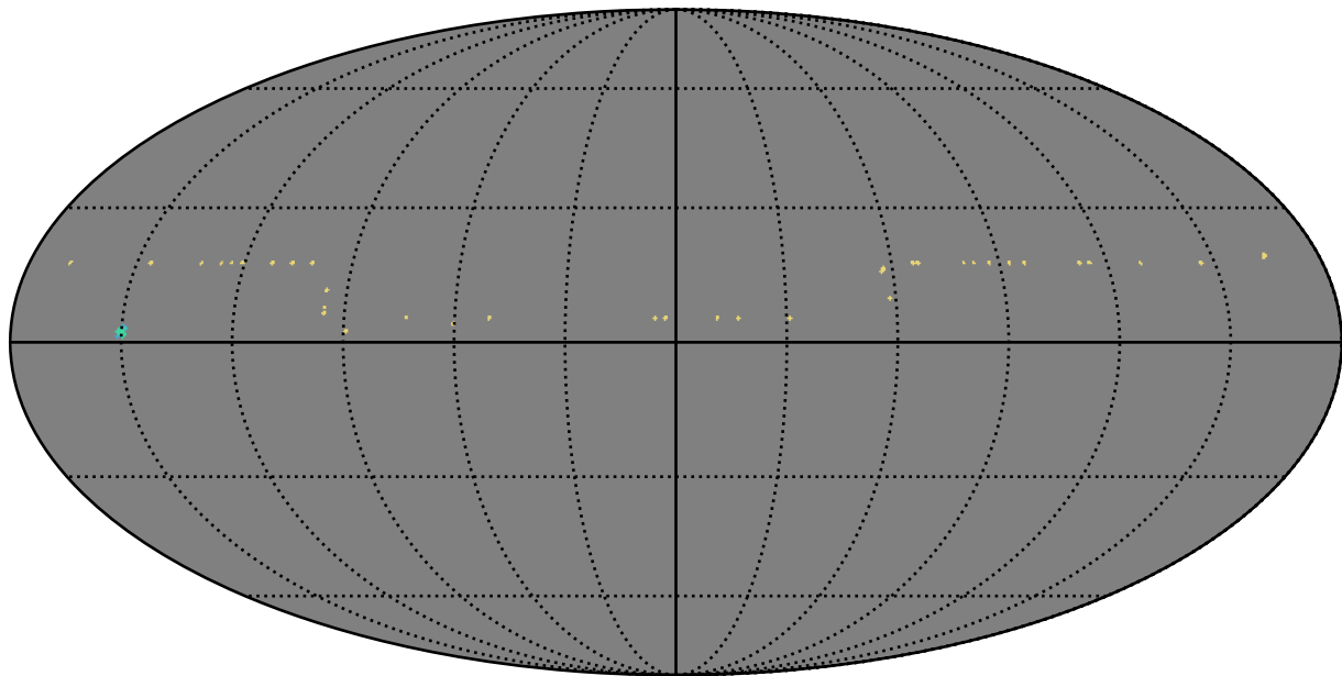
mw_roll_all_v3.3_10yrs y band: AGN_TimeLag_5_days
