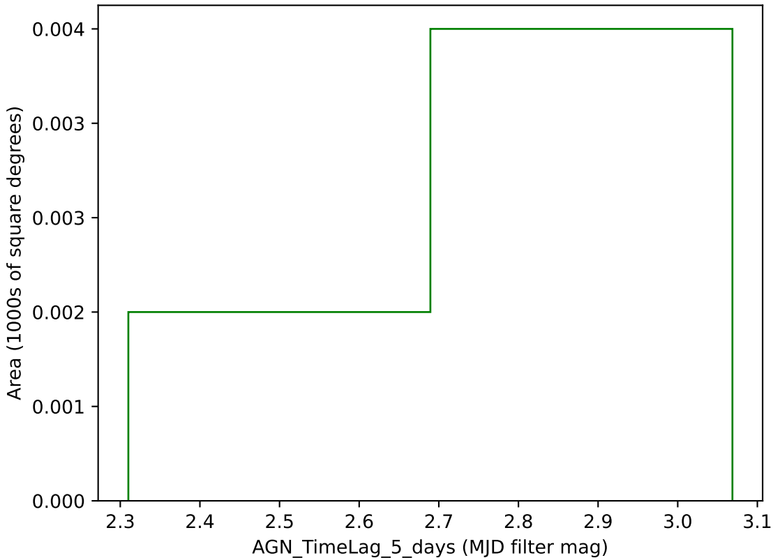
mw_roll_all_v3.3_10yrs g band: AGN_TimeLag_5_days
