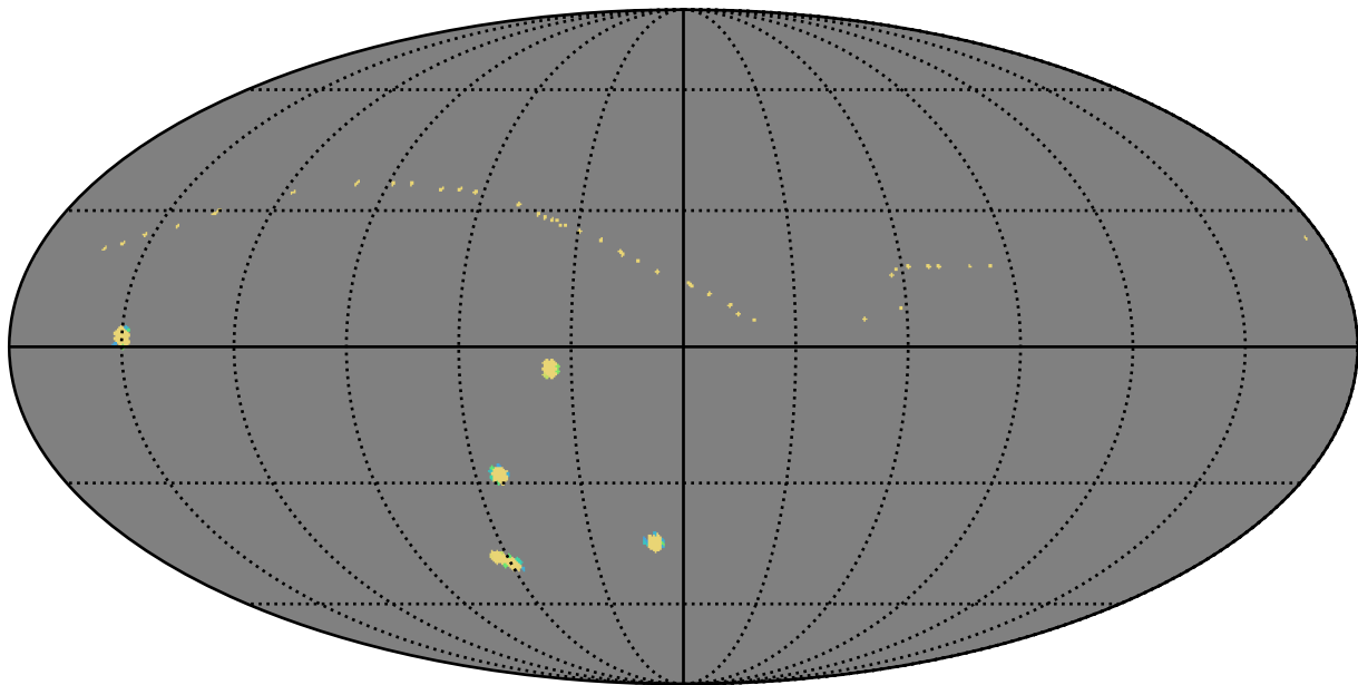
mw_roll_all_v3.3_10yrs all bands: AGN_TimeLag_5_days
