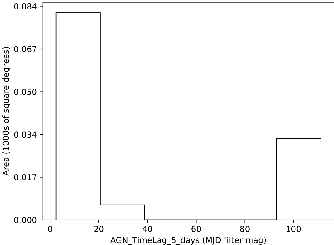
mw_roll_all_v3.3_10yrs all bands: AGN_TimeLag_5_days
