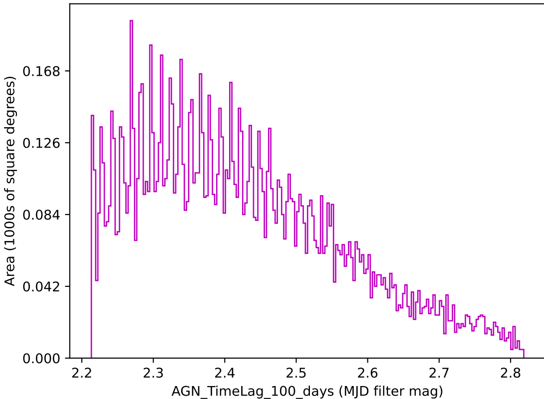
mw_roll_all_v3.3_10yrs z band: AGN_TimeLag_100_days
