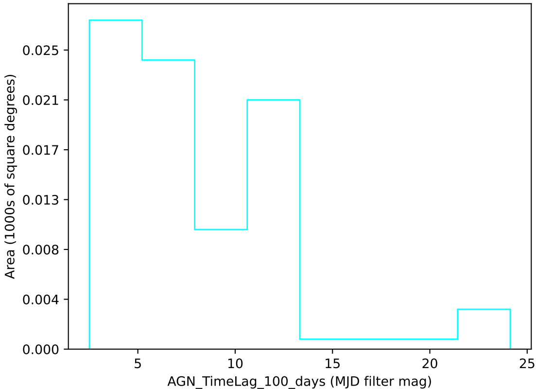
mw_roll_all_v3.3_10yrs u band: AGN_TimeLag_100_days
