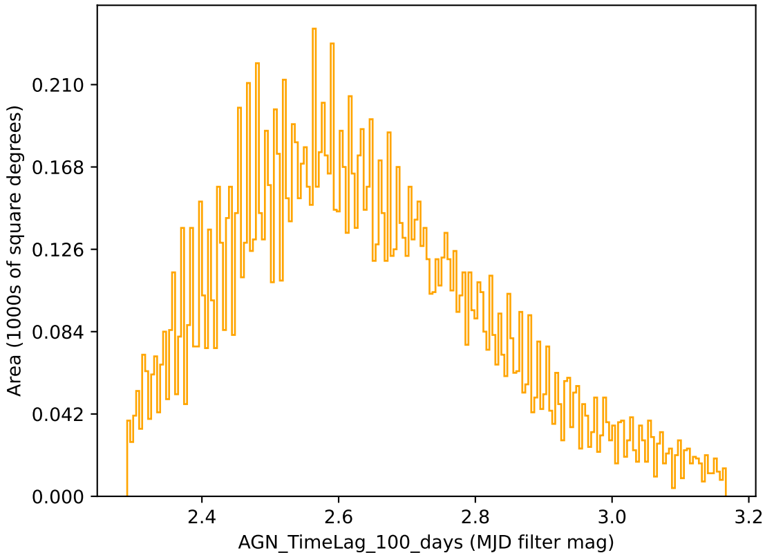
mw_roll_all_v3.3_10yrs r band: AGN_TimeLag_100_days
