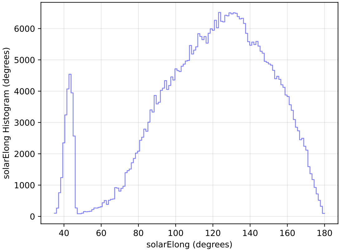
mw_roll_all_v3.3_10yrs WFD z band: solarElong Histogram
