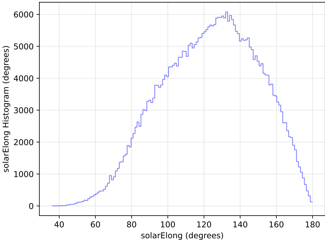
mw_roll_all_v3.3_10yrs WFD y band: solarElong Histogram
