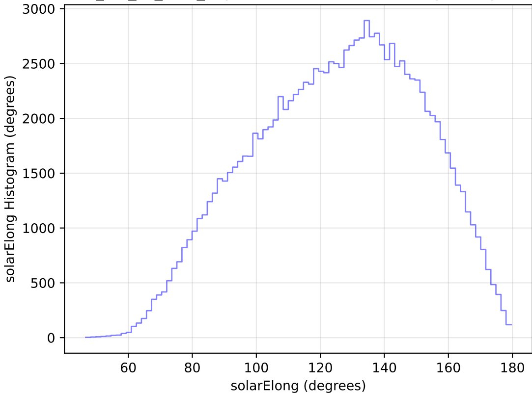
mw_roll_all_v3.3_10yrs WFD u band: solarElong Histogram
