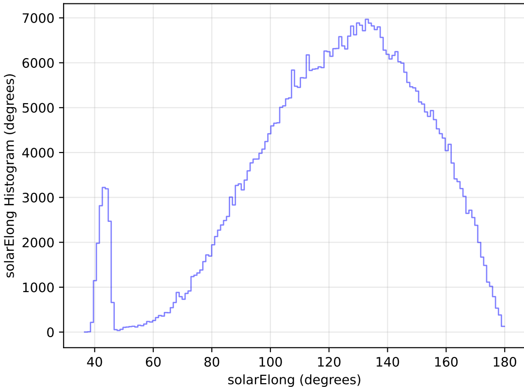
mw_roll_all_v3.3_10yrs WFD r band: solarElong Histogram
