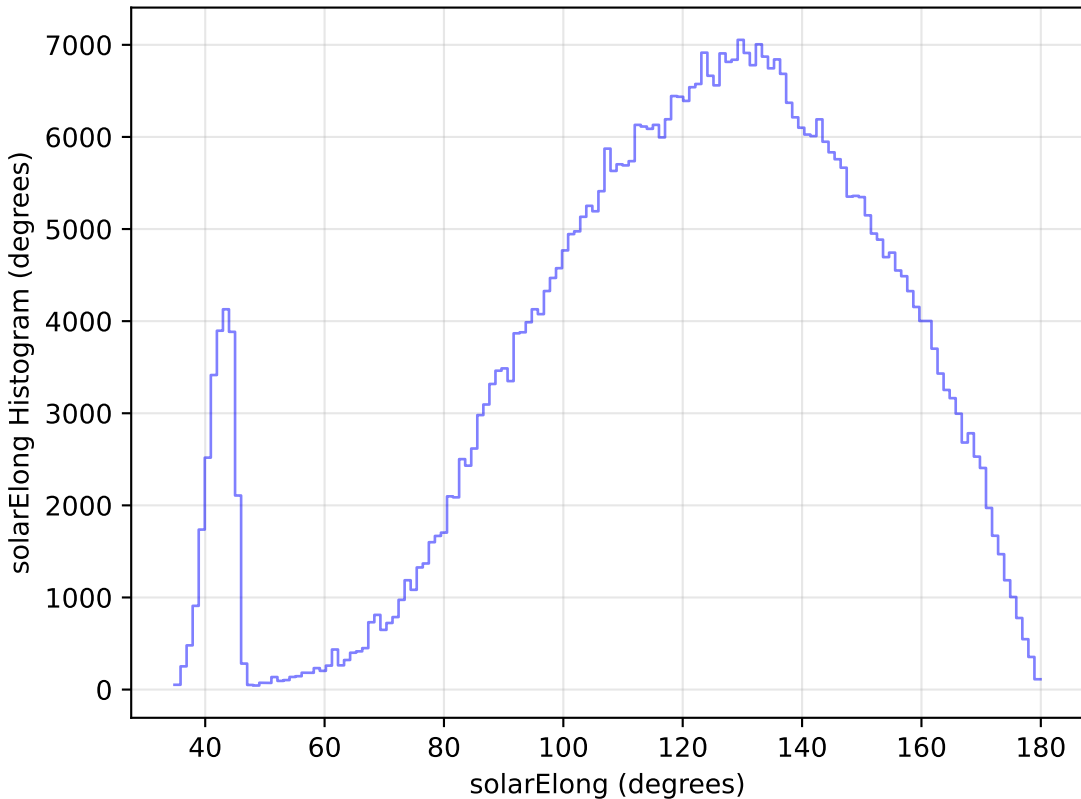
mw_roll_all_v3.3_10yrs WFD i band: solarElong Histogram
