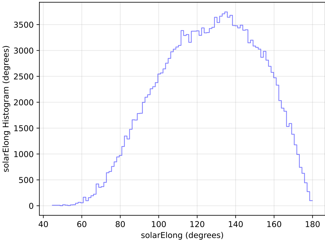
mw_roll_all_v3.3_10yrs WFD g band: solarElong Histogram
